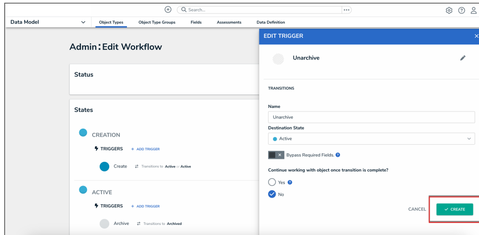
Create Button
