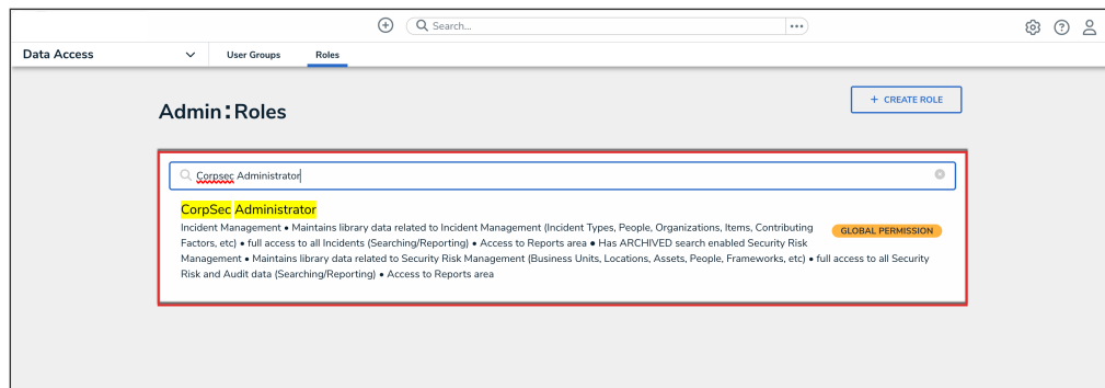
Search Roles
