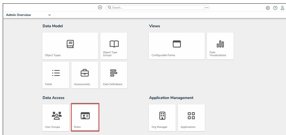
Roles Tile
