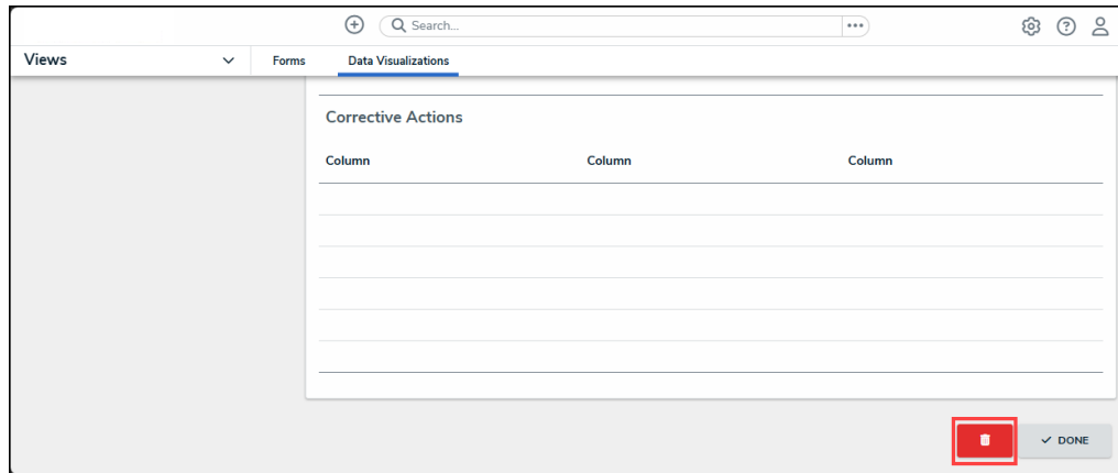
Delete Button
