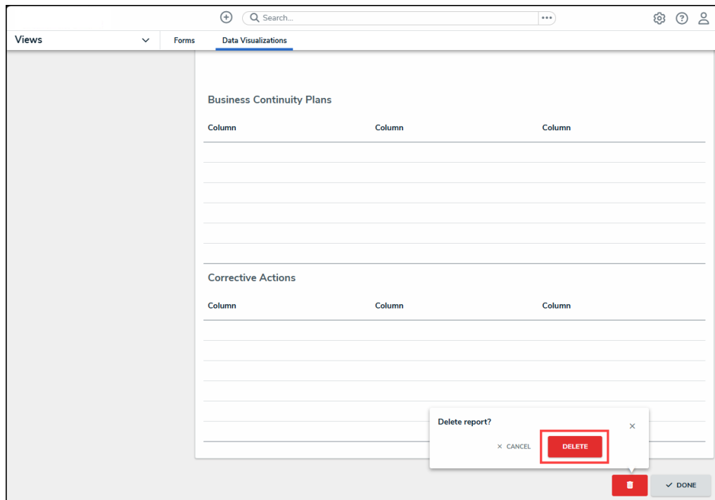
Delete Button
