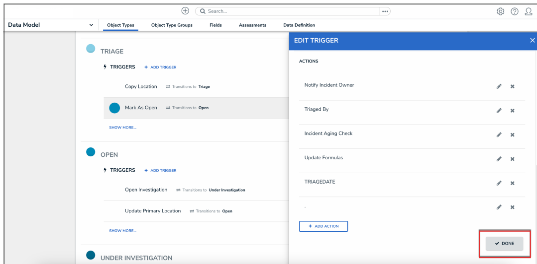
Done Button
