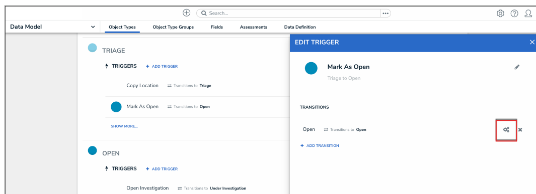
Configure Icon
