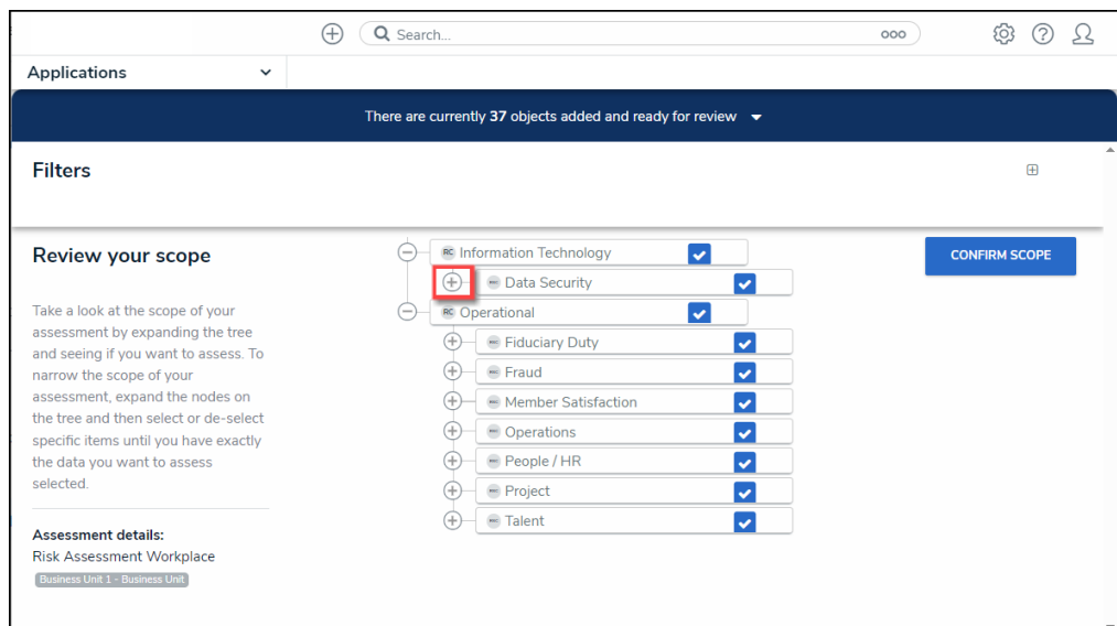
Expand Icon
