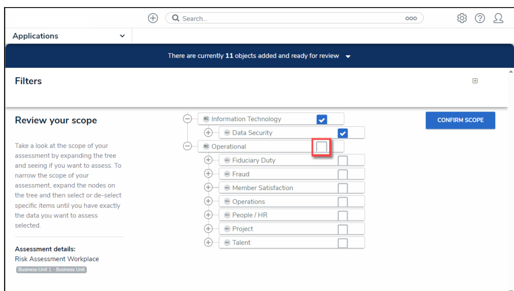
Object Checkbox
