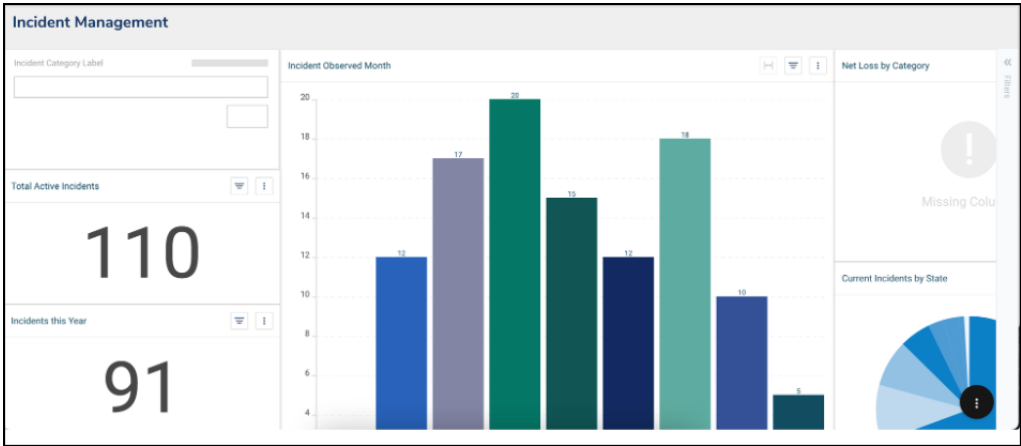
Dashboard
