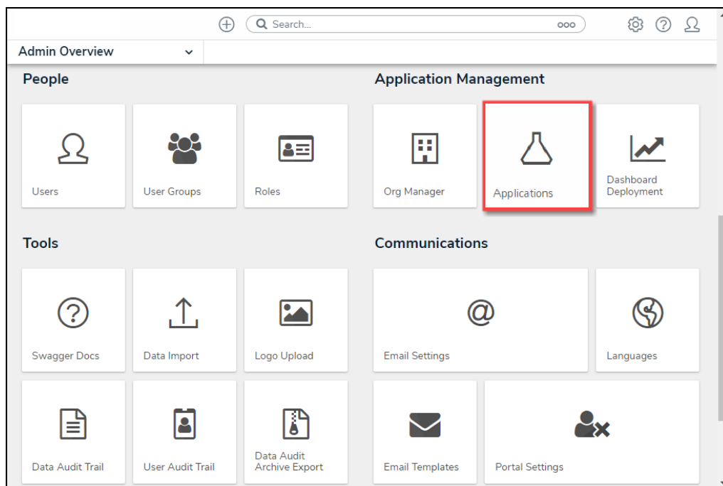
Applications Tile
