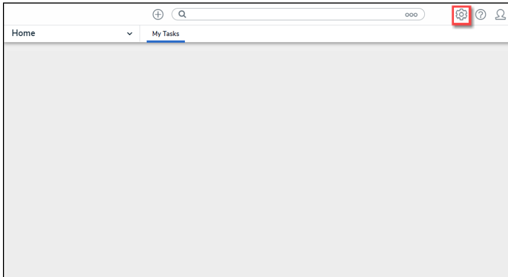
System Icon
