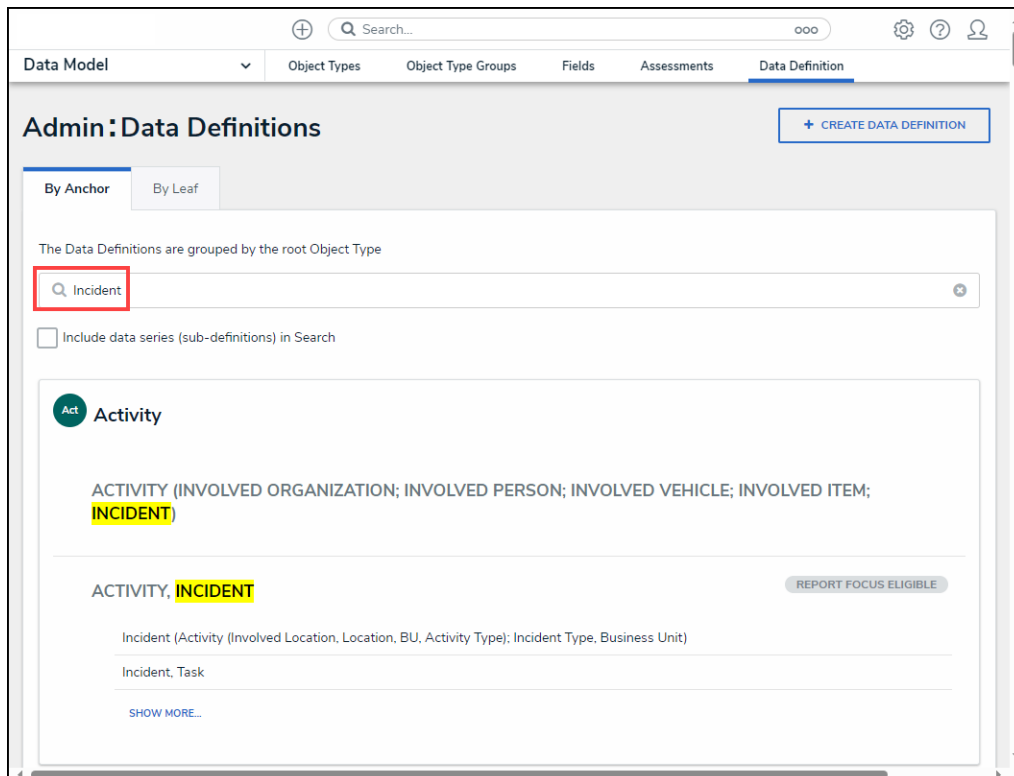
Search Field
