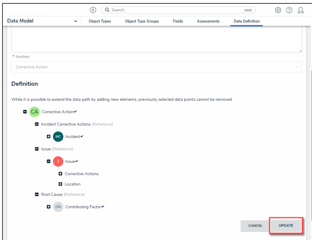
Update Button
