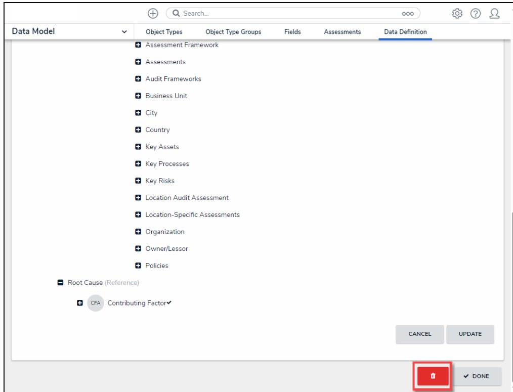
Delete Button
