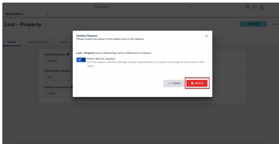
Delete Button
