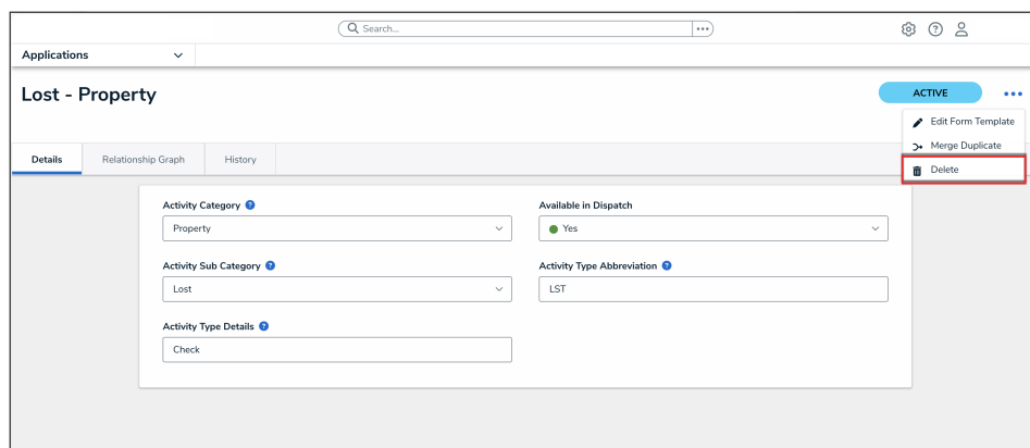
Delete
